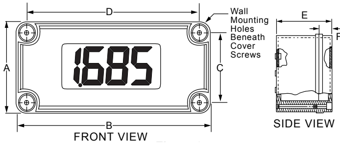
Figure 7: Dimensions and Wall Mounting Information
